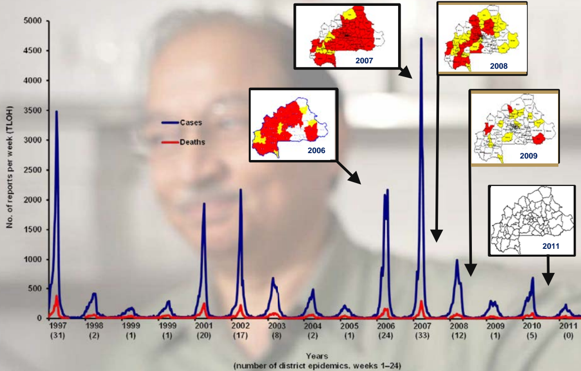
Meningitis Epidemic Curve 1997-2011 (Burkina Faso data)
